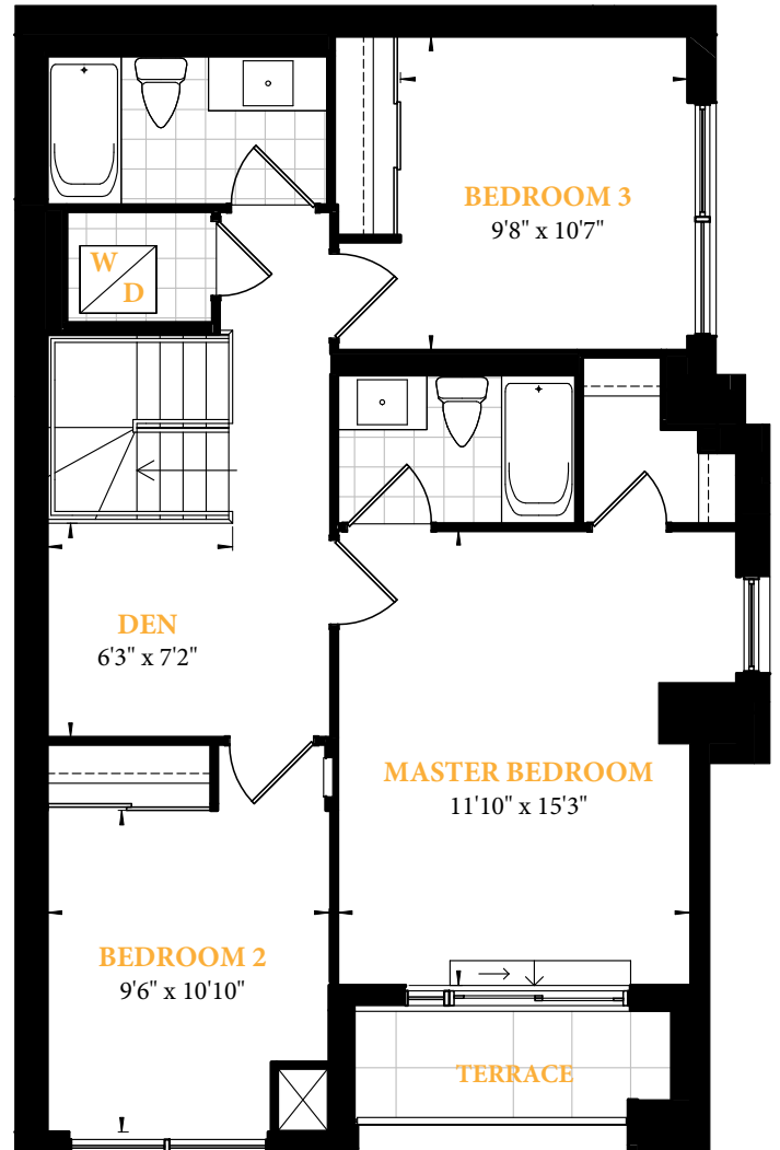
Level 2 (Upper)
