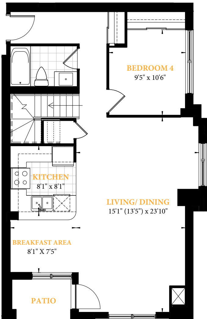
Level 1 (Lower)
